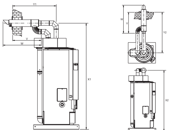
Wall duct concentric
